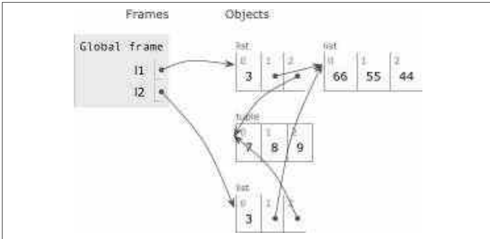
Figure 6-3. Program state immediately after the assignment l2 = list(l1) in Example 6-6. l1 and l2 refer to distinct lists, but the lists share references to the same inner list object [66, 55, 44] and tuple (7, 8, 9) . (Diagram generated by the Online Python Tutor.)
